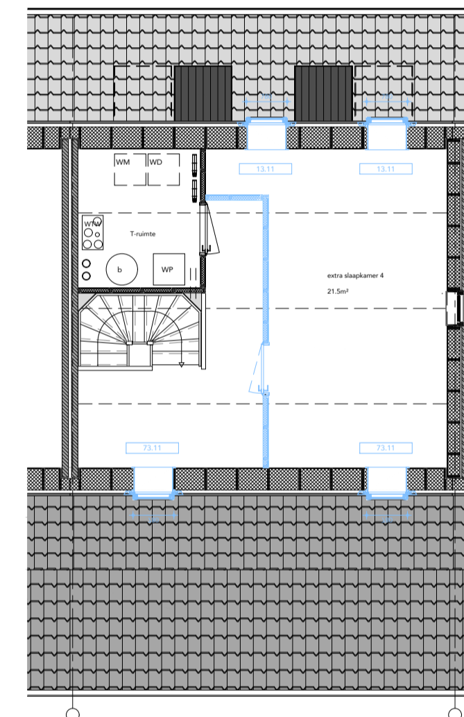
ZOLDERVERDIEPING
