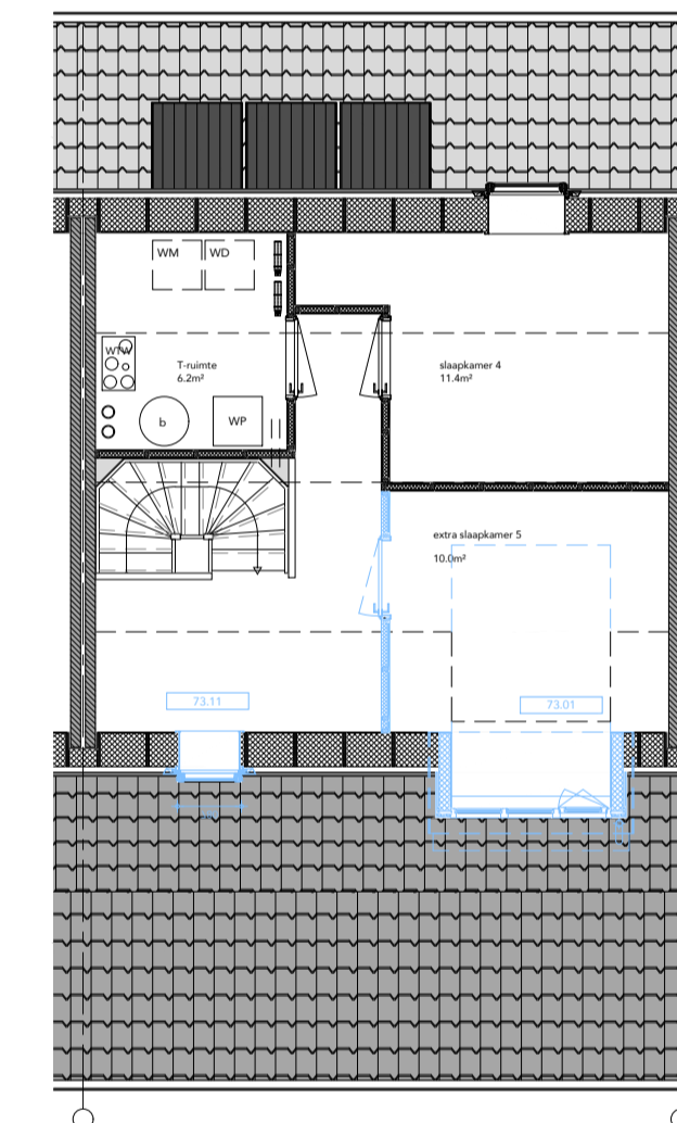
ZOLDERVERDIEPING
