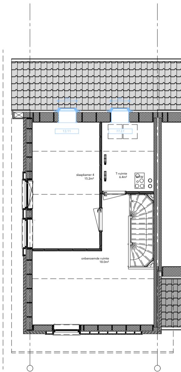
TWEDE VERDIEPING 13.11 dakraam type Velux GGL-MK04 ca.78x98cm
