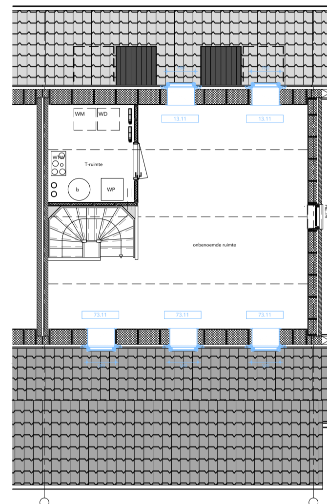
ZOLDERVERDIEPING
