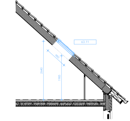
DOORSNEDE 63.11 dakraam type Velux GGL-MK04 ca.78x98cm
