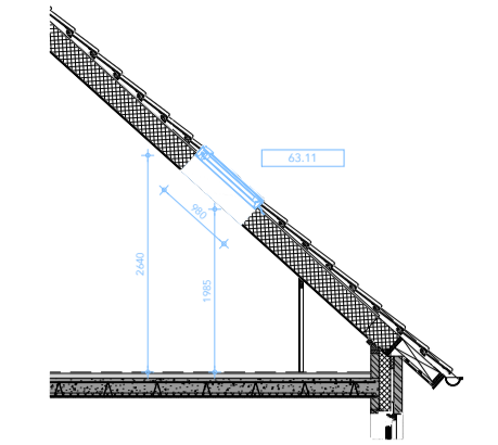
DOORSNEDE 63.11 dakraam type Velux GGL-MK04 ca.78x98cm
