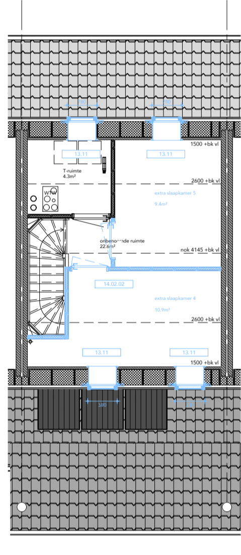
ZOLDERVERDIEPING
