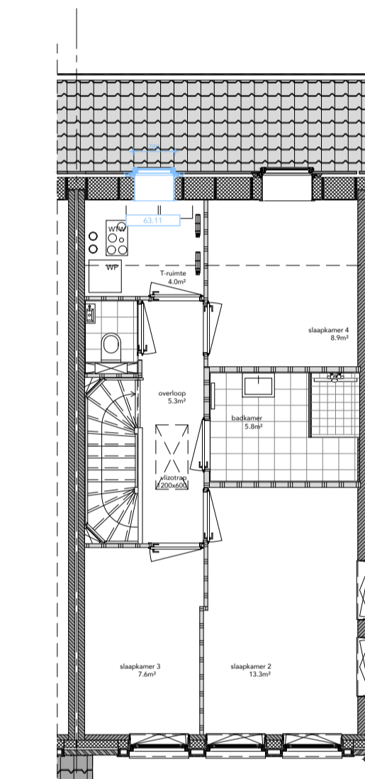
TWEDE VERDIEPING 63.11 dakraam type Velux GGL-MK04 ca.78x98cm
